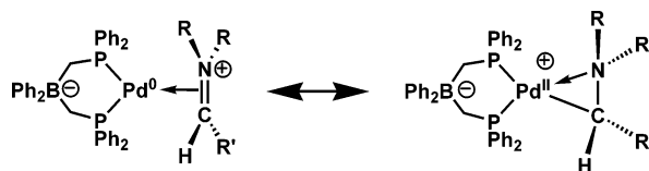
Figure 4. Limiting resonance forms for the palladacycles.
