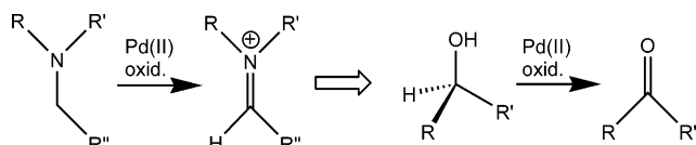
Figure 1. Relationship between amine-to-iminium ion and alcohol-to-ketone oxidation reactions.
